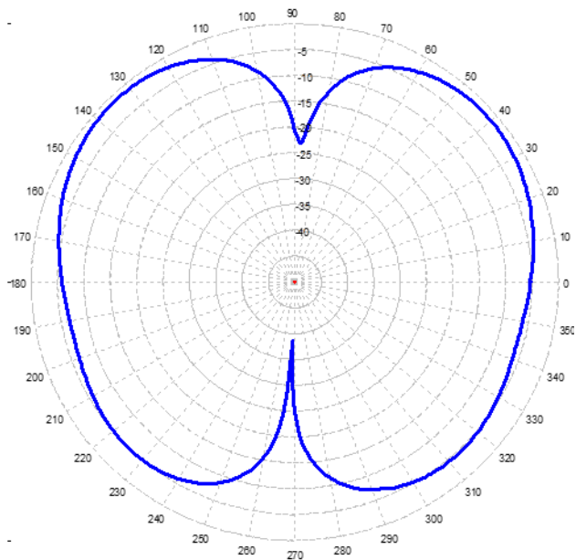
450 MHz
