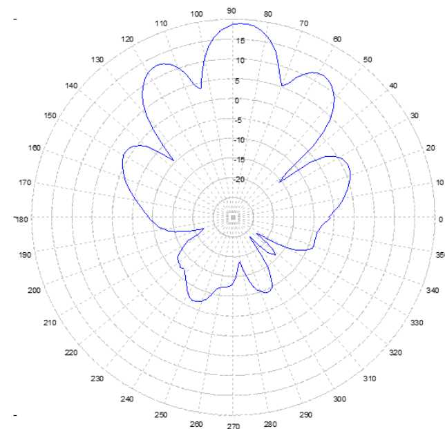
2500 MHz
