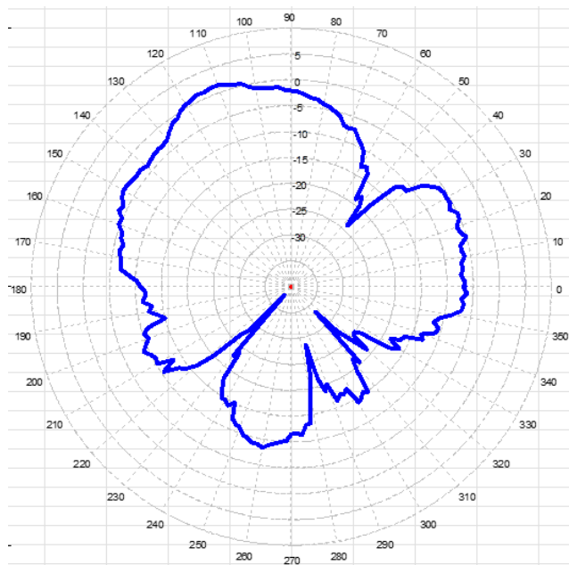
5.7 MHz
