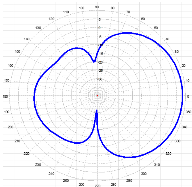
370 MHz
