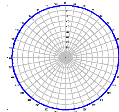
866 MHz Azimuth
