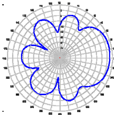
902 MHz Azimuth
