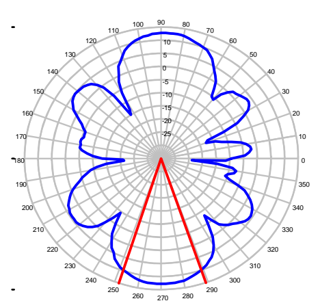
Azimuth Plot @ 5924 MHz
