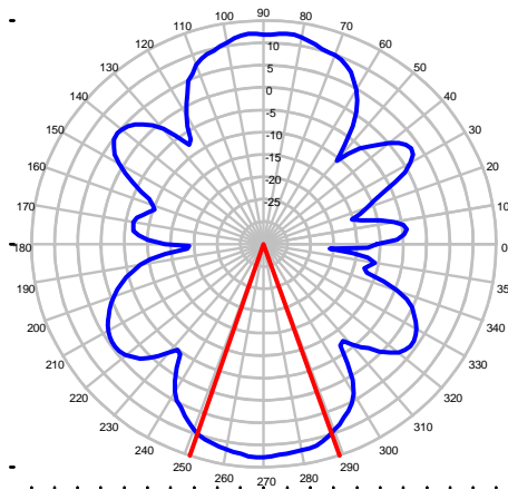
Azimuth Plot @ 5776 MHz
