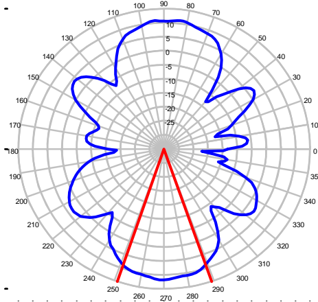
Azimuth Plot @ 5726 MHz
