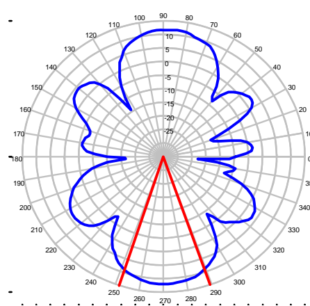
Azimuth Plot @ 5876 MHz
