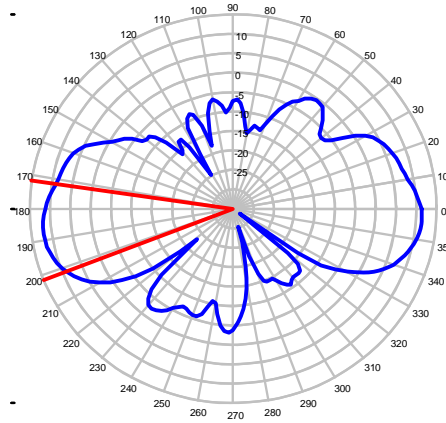
Elevation Plot @ 5776 MHz
