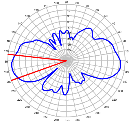
Elevation Plot @ 5876 MHz
