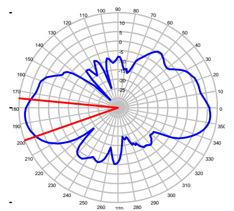
Elevation Plot @ 5924 MHz
