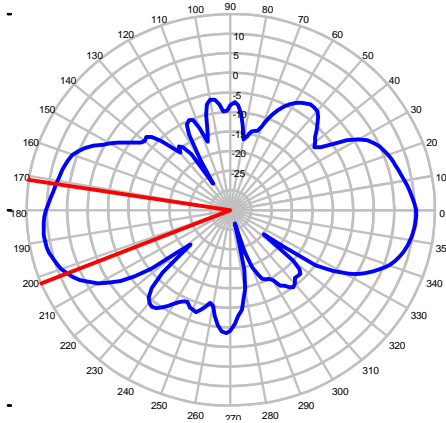
Elevation Plot @ 5726 MHz
