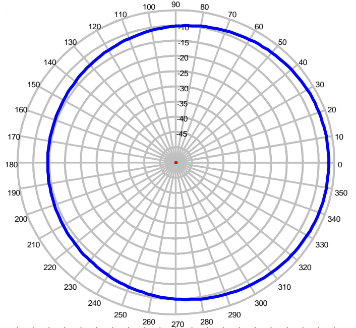
460 MHz – Azimuth
