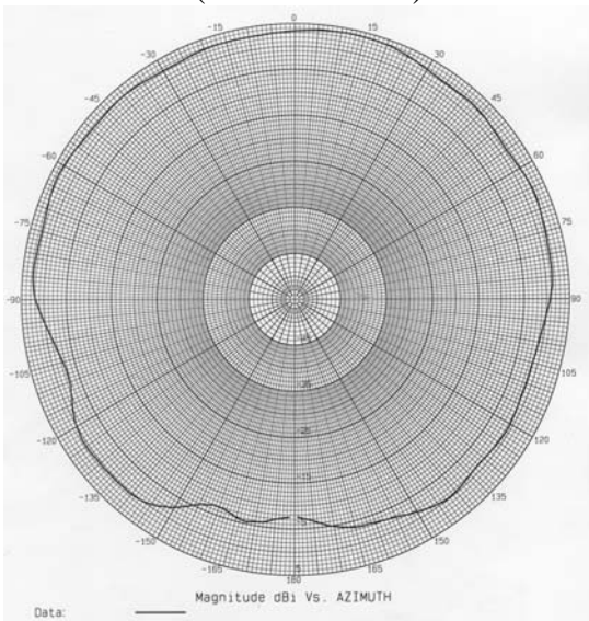
CMD @ 2500 MHz – Azimuth Plot (Element 1 of 3)
