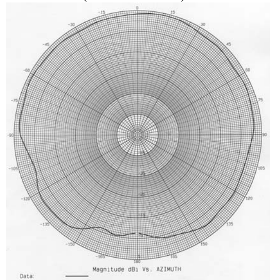
CMD @ 3500 MHz- Azimuth Plot (Element 1 of 3)
