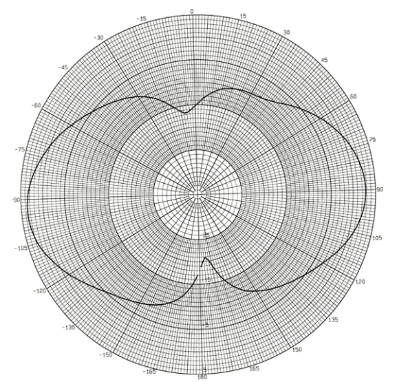
Elevation Plot 2200 - 2700 MHz
