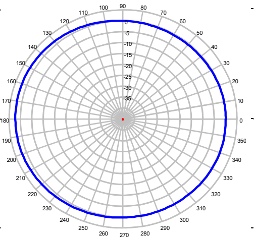
1850 MHz – Azimuth Plot
