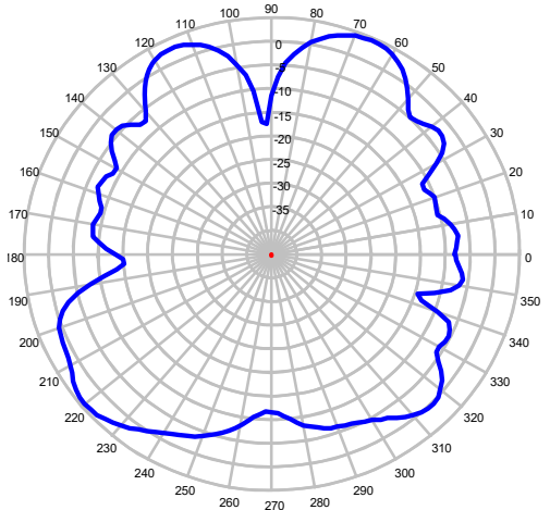
2700 MHz – Elevation Plot
