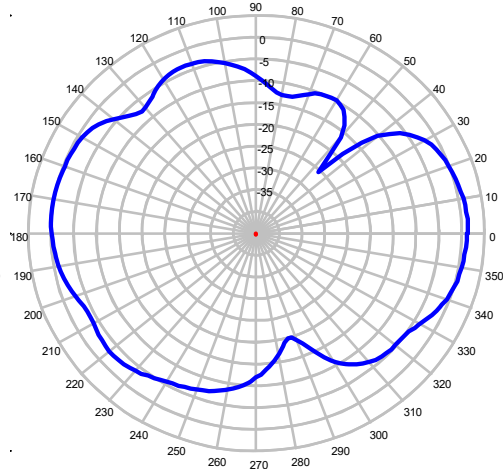
1900 MHz – Elevation Plot
