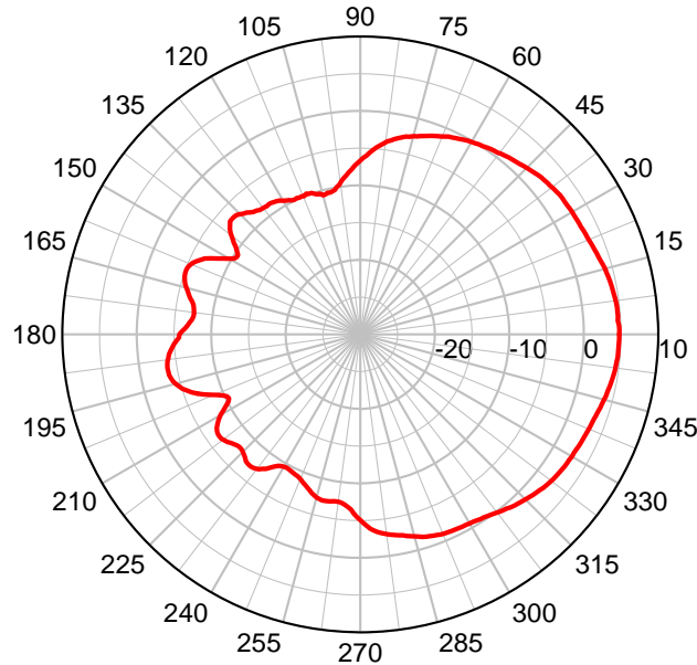
EM-2400 – Elevation Plot
