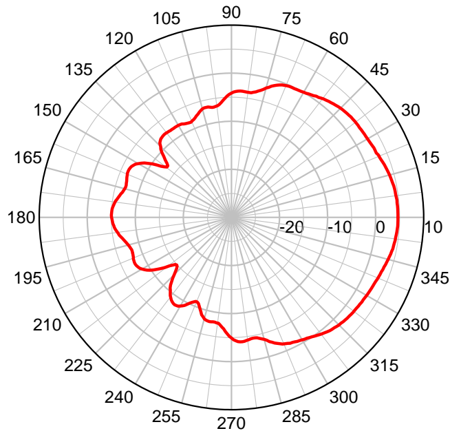
EM-2400 – Azimuth Plot
