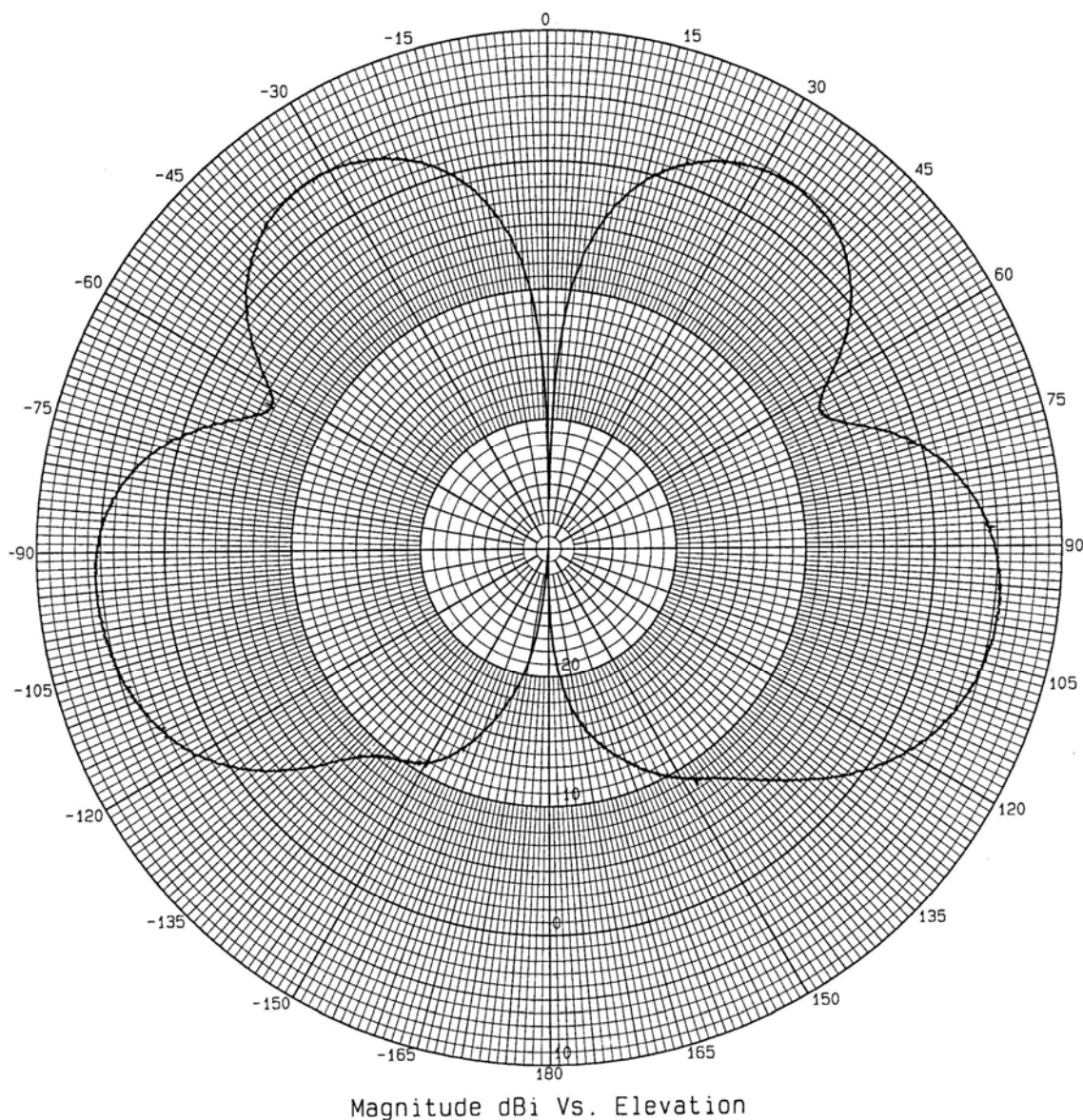
IMAG5-1350 – Elevation Plot
