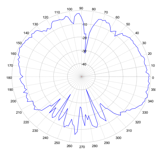
5925 MHz – Elevation Plot
