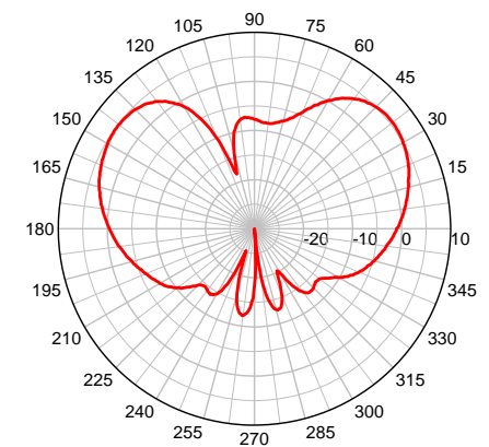
MGW 2400 MHz – Elevation Plot
