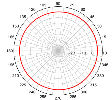
MGW 2400 MHz – Azimuth Plot
