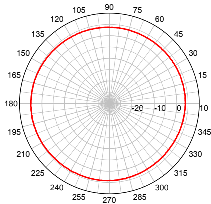
MGW 1900 MHz – Azimuth Plot
