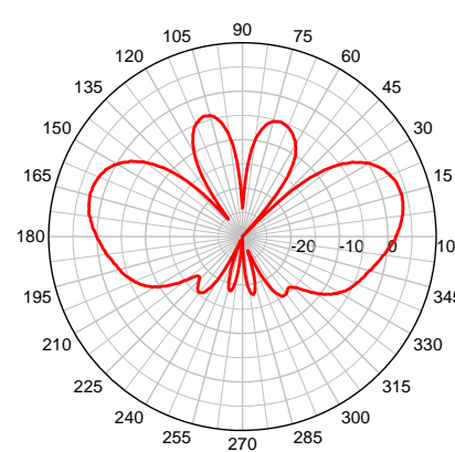
MGW 2400 MHz – Elevation Plot
