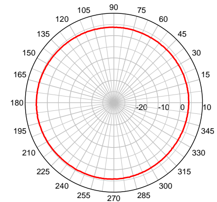
MGW 1900 MHz – Azimuth Plot
