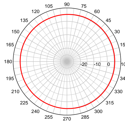
MGW 2400 MHz – Azimuth Plot
