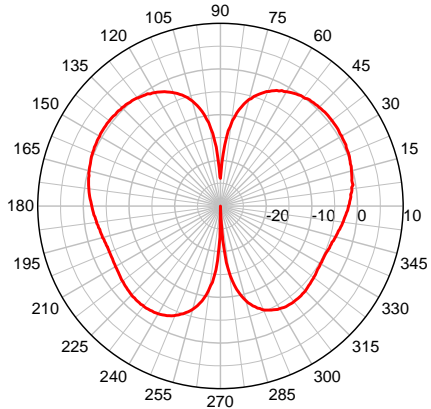
MGW 900 MHz Band – Elevation Plot
