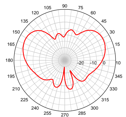
MGW 1900 MHz – Elevation Plot
