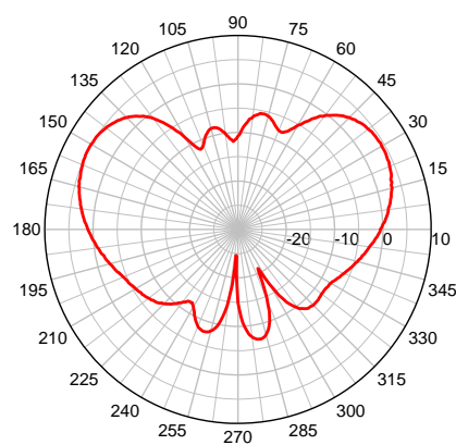
MGW 1900 MHz – Elevation Plot
