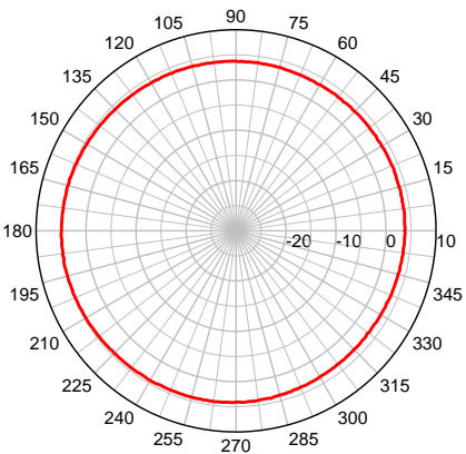
MGW 1900 MHz – Azimuth Plot
