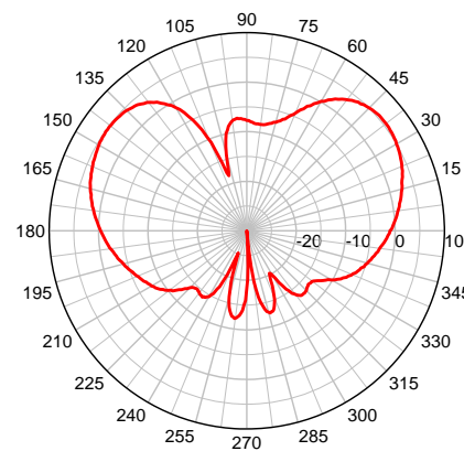
MGW 2400 MHz – Elevation Plot
