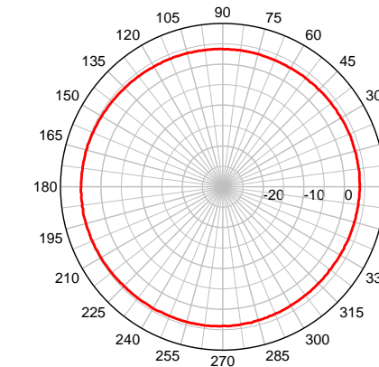
SMW 1.7 to 2.7 GHz – Azimuth Plot
