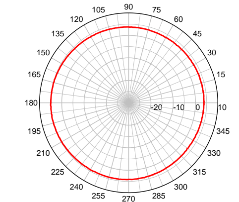
SMW 1.7 to 2.7 MHz – Azimuth Plot
