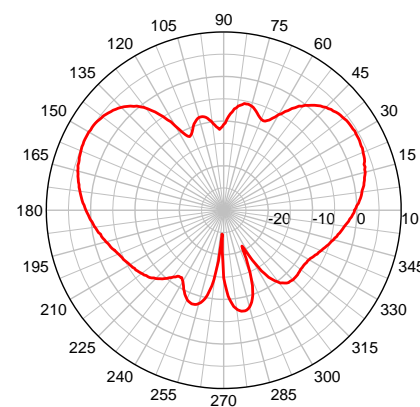
SMW 1.7 to 2.7 GHz – Elevation Plot
