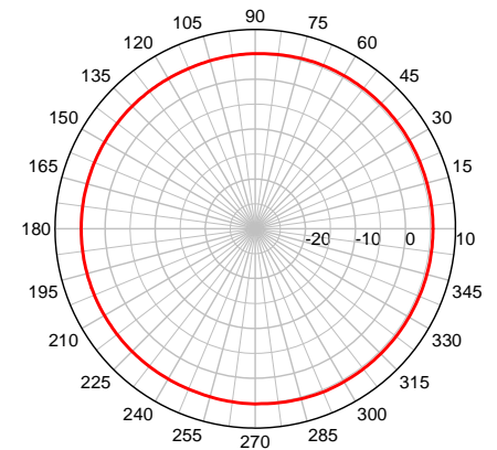
Cable #3 MGW 2000 MHz – Azimuth Plot
