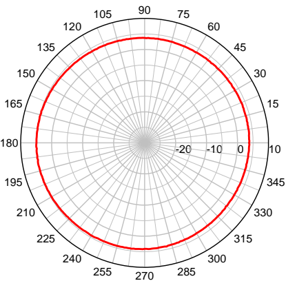
Cable #2 MGW 2400 MHz – Azimuth Plot
