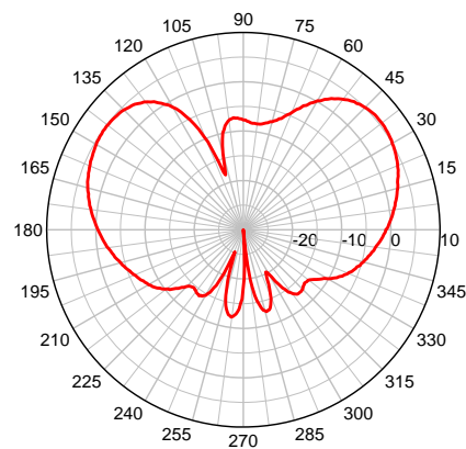
Cable #2 MGW 2400 MHz – Elevation Plot
