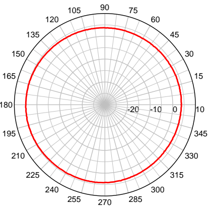
Cable #1 MGW 1900 MHz – Azimuth Plot
