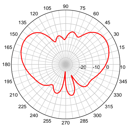
Cable #1 MGW 1900 MHz – Elevation Plot
