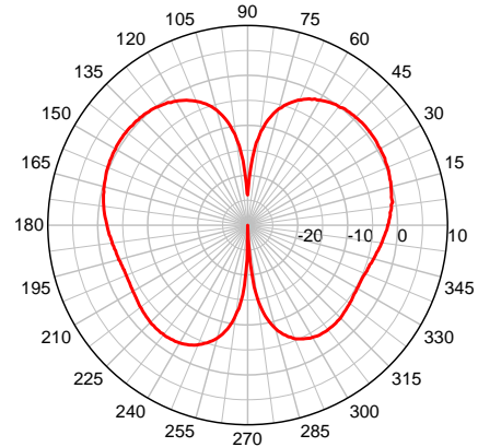
Cable #1 MGW 900 MHz Band – Elevation Plot
