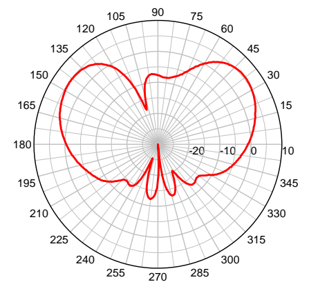
Cable #3 MGW 2000 MHz – Elevation Plot
