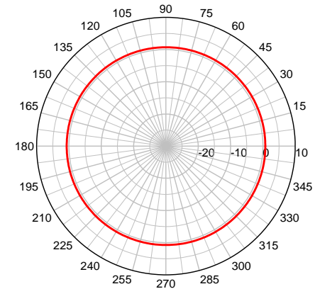
Cable #1 MGW 900 MHz Band – Azimuth Plot
