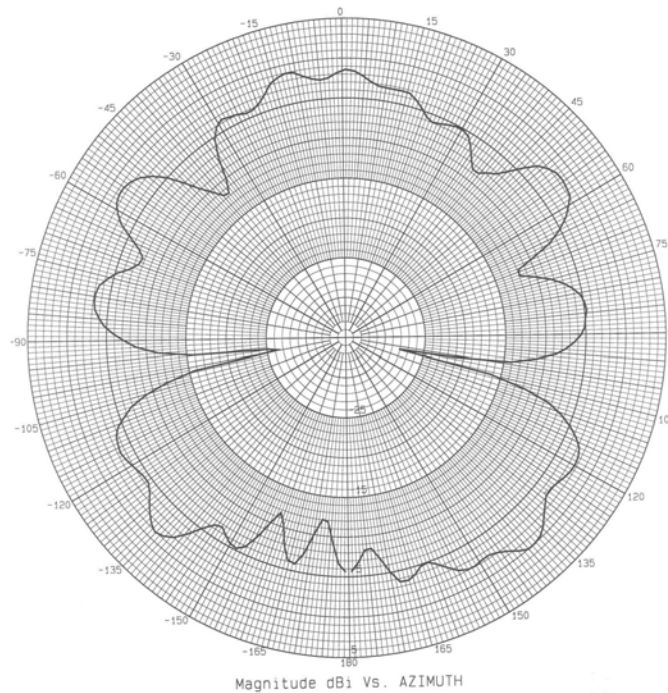
MGW303 Azimuth Plot @ 5.9 GHz
