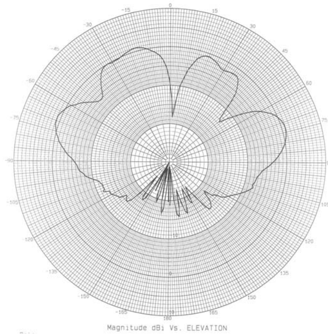
MGW303 Elevation Plot @ 5.9 GHz
