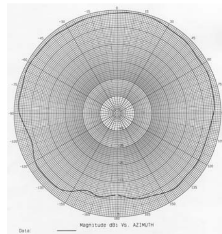
MSMD @ 3500 MHz – Azimuth Plot
