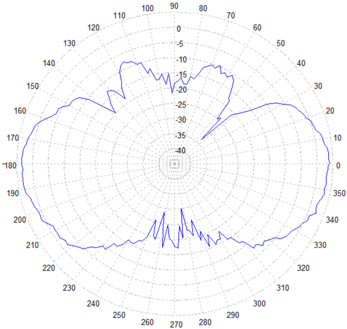
LTE – 3.55 GHz - Elevation Plot
