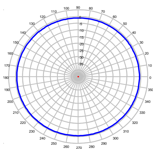
850 MHz – Azimuth Plot
