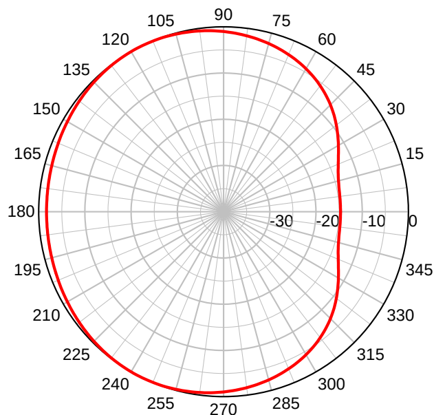
ODR-2400T180K – Azimuth Plot
