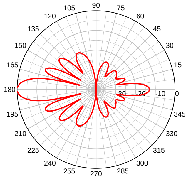
ODR-2400T180K – Elevation Plot
