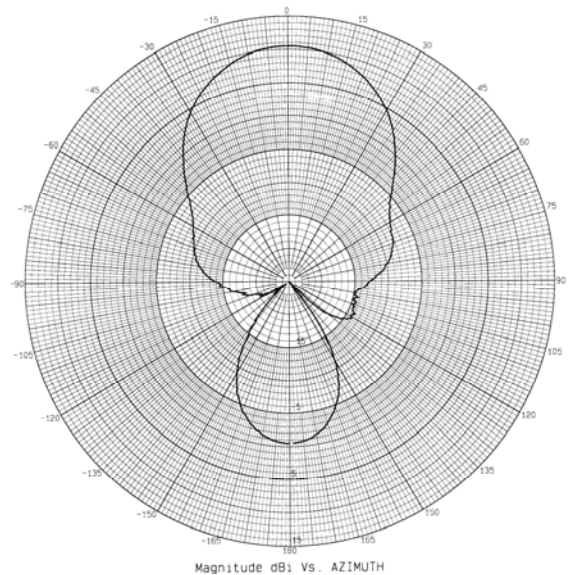
PN10-3000 @ 3.5 GHz – Azimuth Plot
