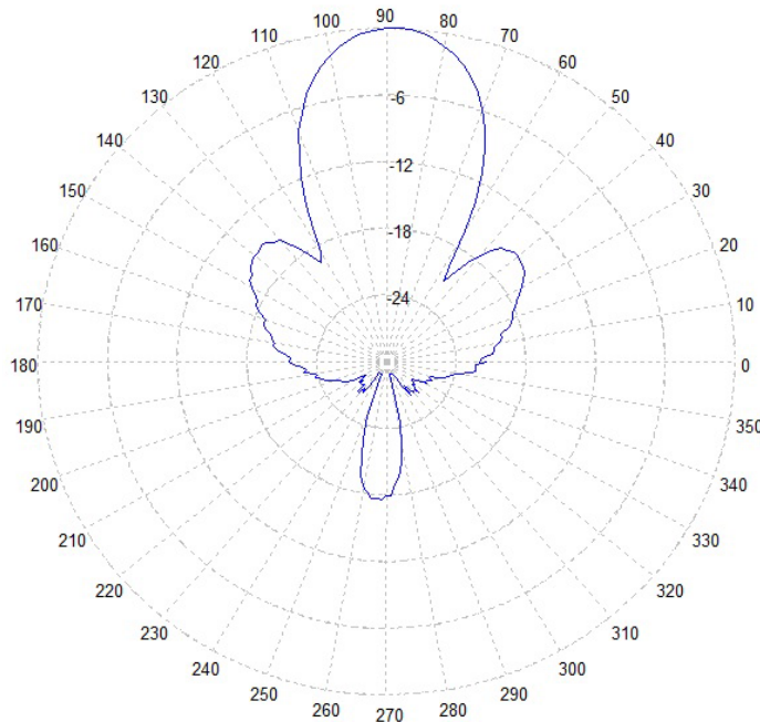
PN17-2400 @ 2450 MHz -Azimuth
