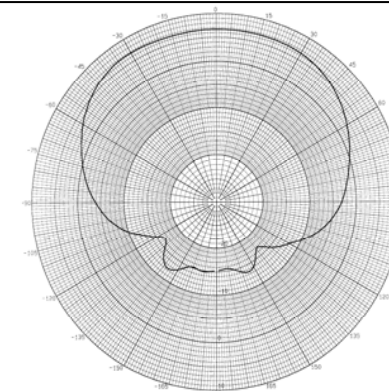
Azimuth Plot @ 2500 MHz
