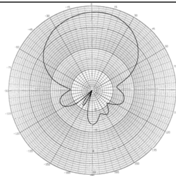
Azimuth Plot @ 2450 MHz
