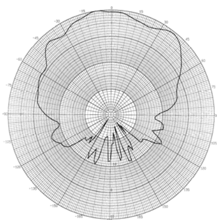
Azimuth Plot @ 4900 MHz
