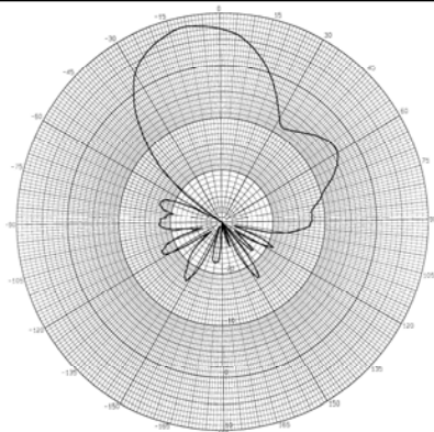
Azimuth Plot @ 4900 MHz
