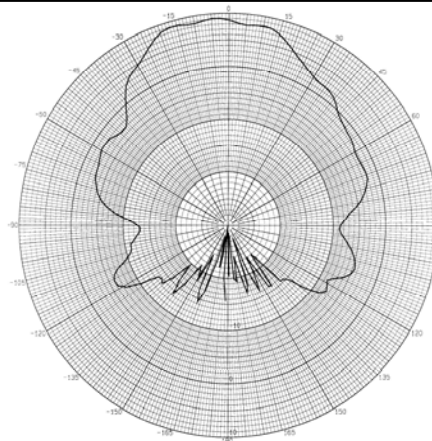
Azimuth Plot @ 5400 MHz
