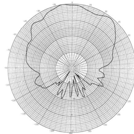
Azimuth Plot @ 5850 MHz
