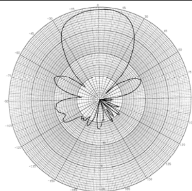
Azimuth Plot @ 5400 MHz
