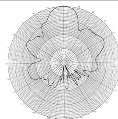
Azimuth Plot @ 5850 MHz
