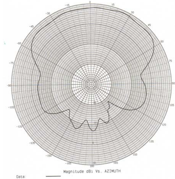
4.9-6.0 GHz – Azimuth Plot
