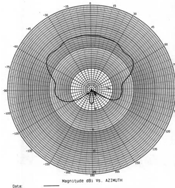
PS10-5500-120 – Azimuth Plot
