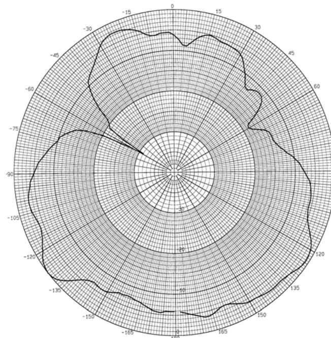
SMW 412 Series at 5950 MHz – Azimuth Plot
