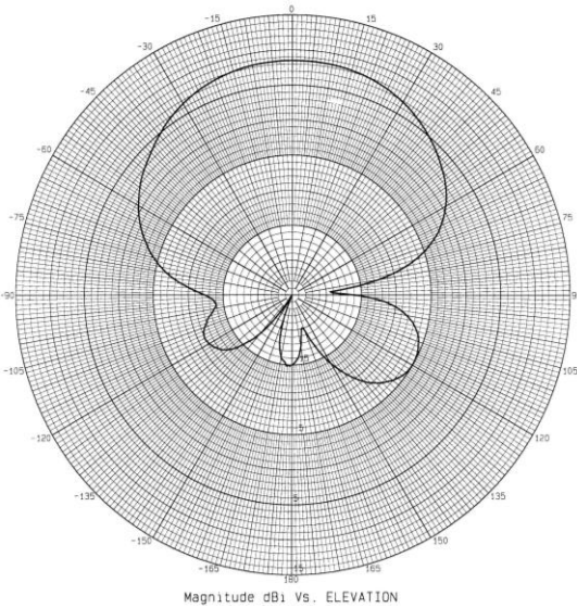
Elevation Plot at 2400 MHz
