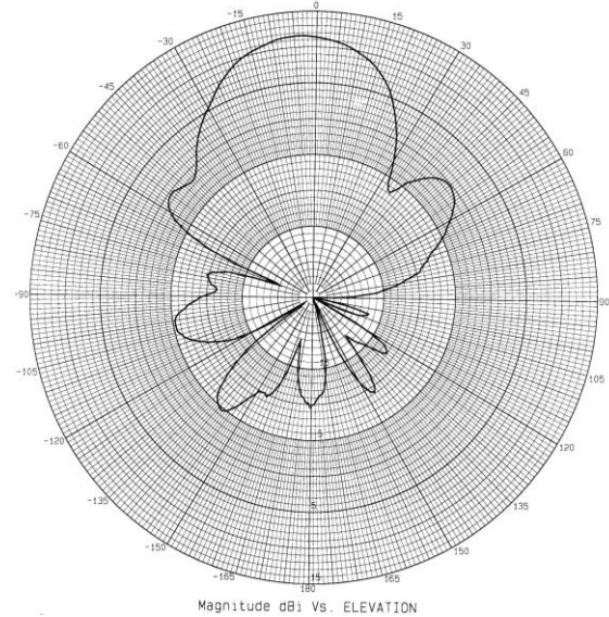
Elevation Plot at 5500 MHz
