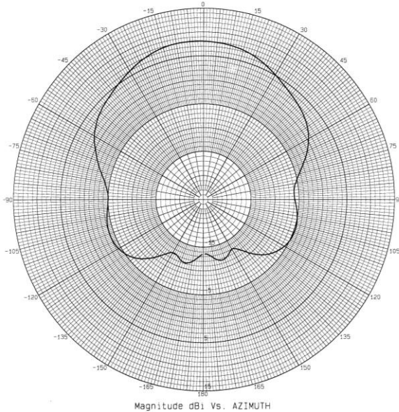
Azimuth Plot at 2400 MHz
