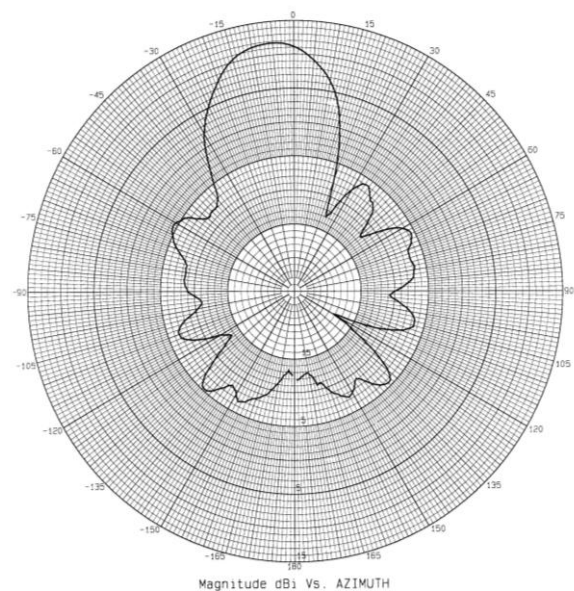
Azimuth Plot at 5500 MHz
