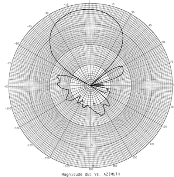
YAG12-5500 @5500 MHz – Azimuth Plot
