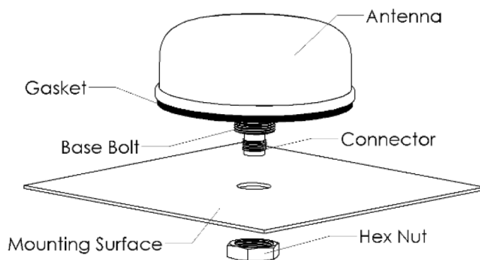
Shown: Surface Mount
