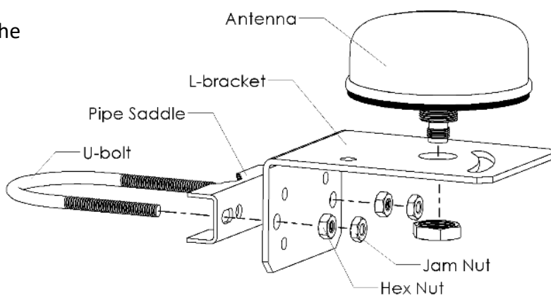
Shown: Optional Pipe Mount
