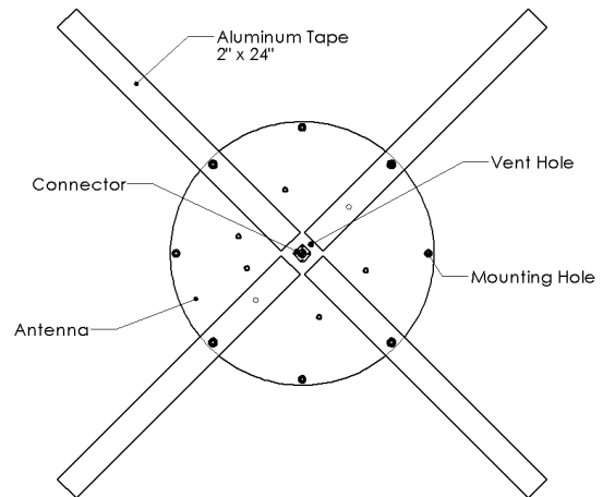
Aluminum tape ground plane layout (FIG 1)
