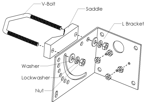
Shown: Mounting Kit and Hardware
