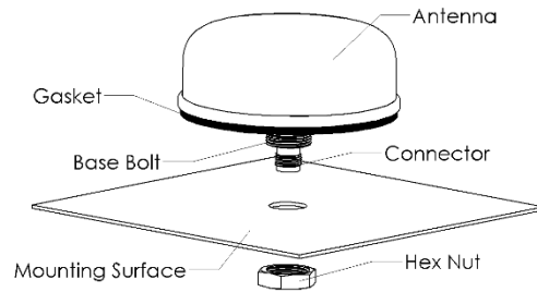
Shown: Surface Mount
