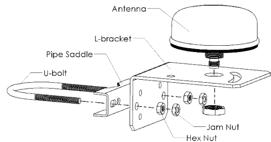
Shown: Optional Pipe Mount
