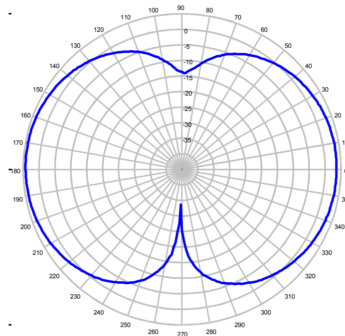
160 MHz – Elevation Plot
