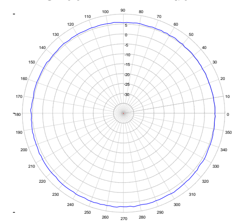
3700 MHz Azimuth
