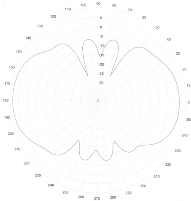
BD-2400 @ 2450 MHz- Azimuth Plot
