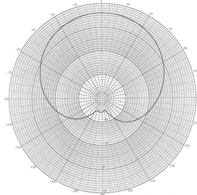
BP6-868LCP @ 868 MHz-Azimuth
