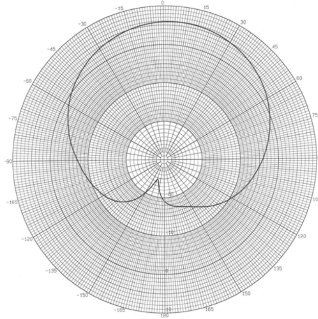
BP6-868LCP @ 868 MHz-Elevation
