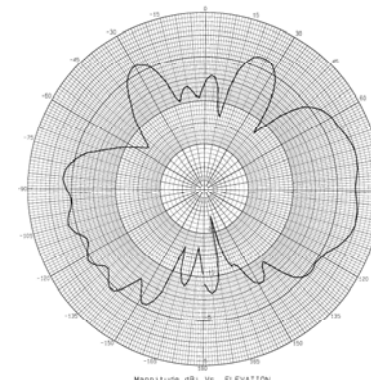
3700 MHz – Elevation Plot
