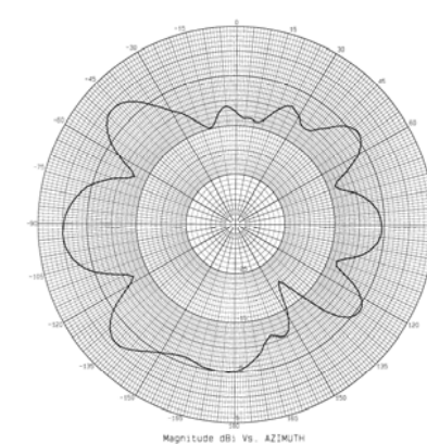
3700 MHz – Azimuth Plot
