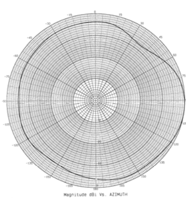
1850 MHz – Azimuth Plot
