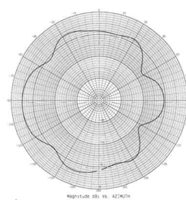
2700 MHz – Azimuth Plot
