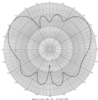
1750 MHz – Elevation Plot
