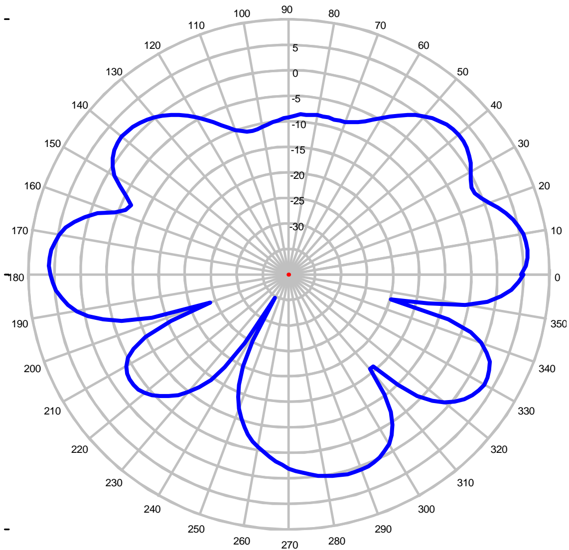
ECO5 @ 915 MHz – Elevation Plot
