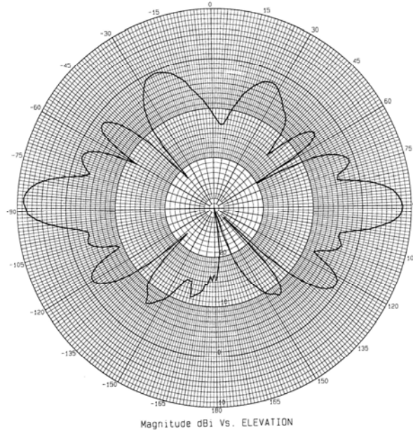
ECOM9-5900 – Elevation Plot
