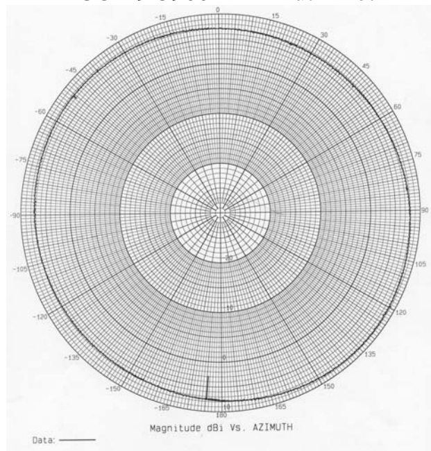
ECOM9-5900 – Azimuth Plot
