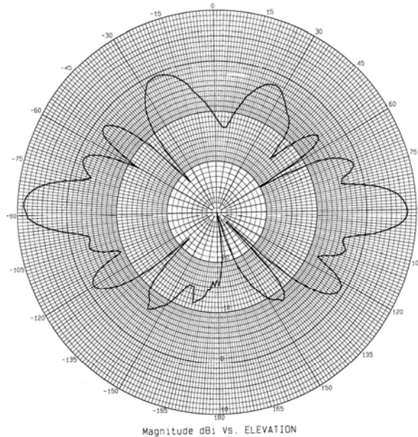
ECO9-5900 – Elevation Plot
