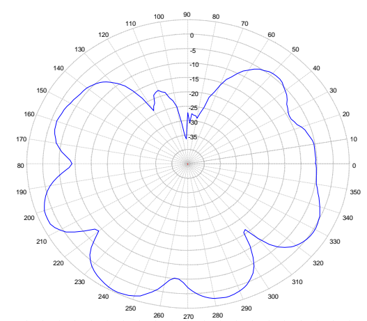
Azimuth Plot at 2700 MHz
