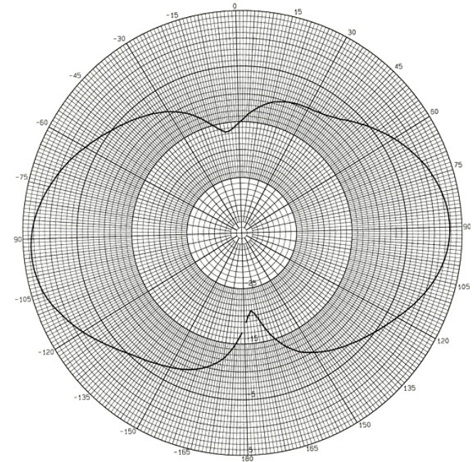
Elevation Plot 2200 - 2500 MHz
