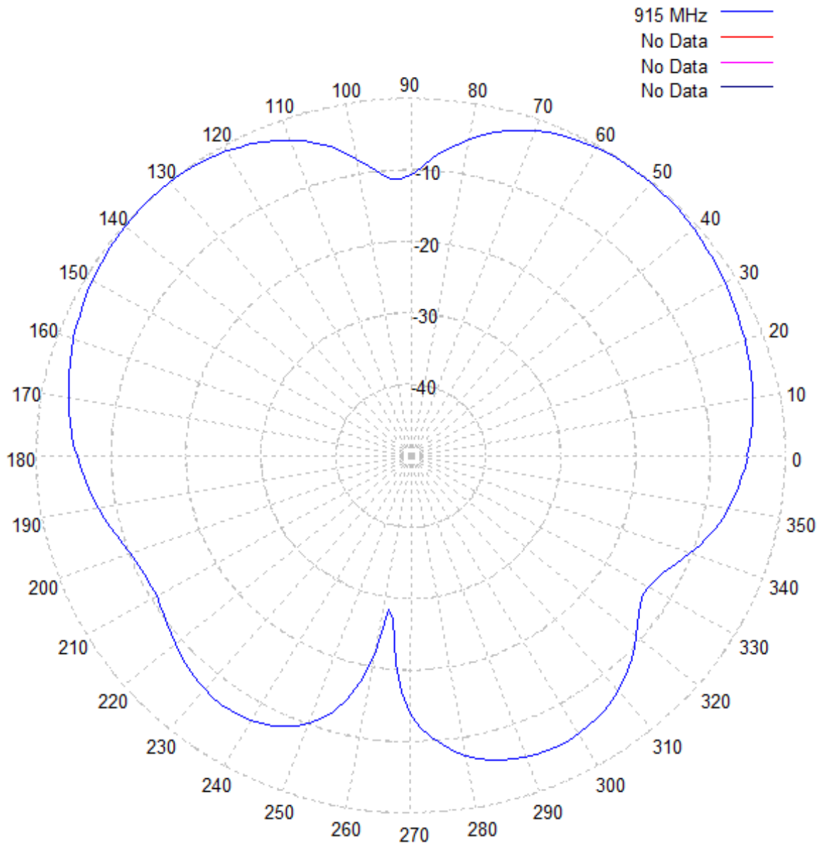
HD3-915 Series- Elevation Plot @ 915 MHz
