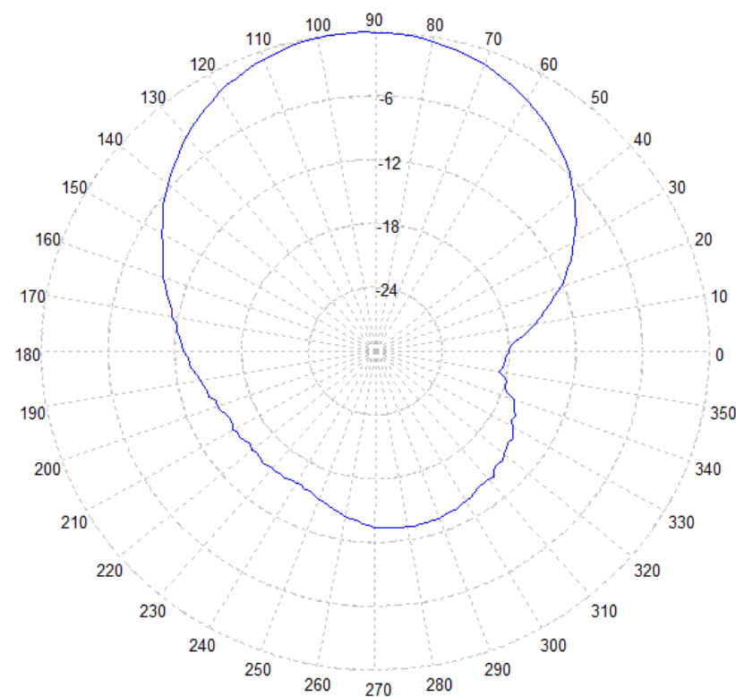
915 MHz – Azimuth Plot
