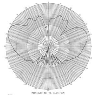
5950 MHz – Elevation
