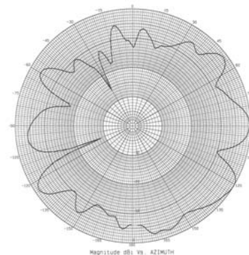
5500 MHz – Azimuth
