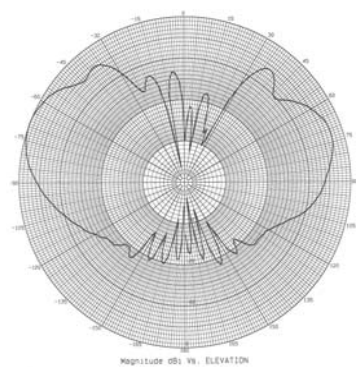
5500 MHz – Elevation
