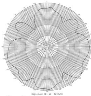
4900 MHz – Azimuth
