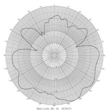
5950 MHz – Azimuth
