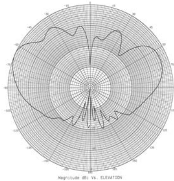
4900 MHz – Elevation
