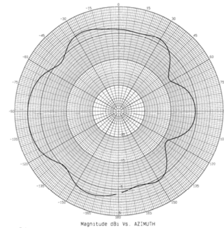
2700 MHz – Azimuth Plot
