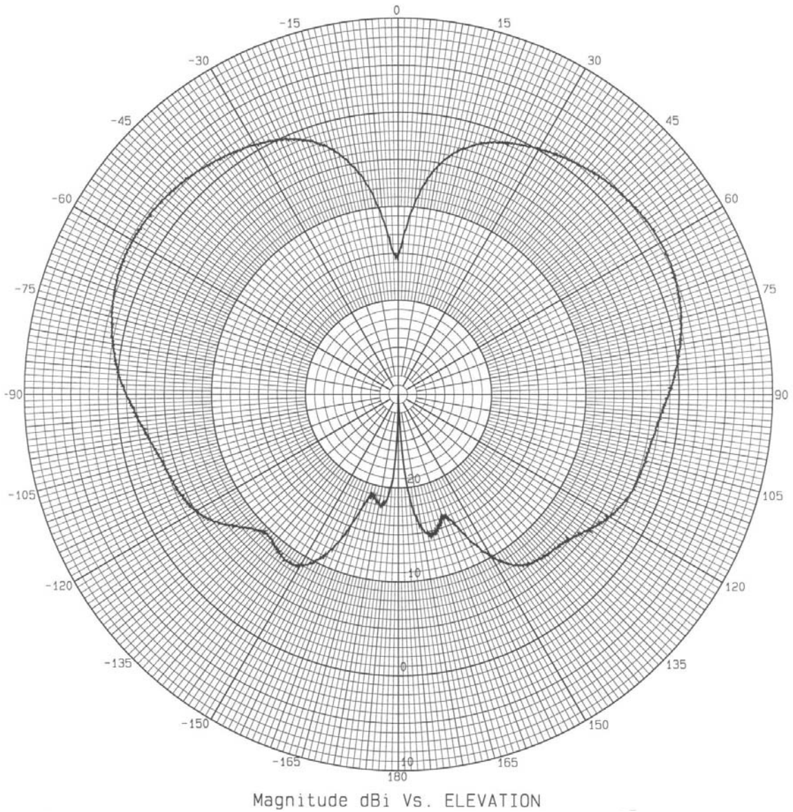
2350 MHz – Elevation Plot
